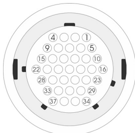
37-way CPC connector - Front view
