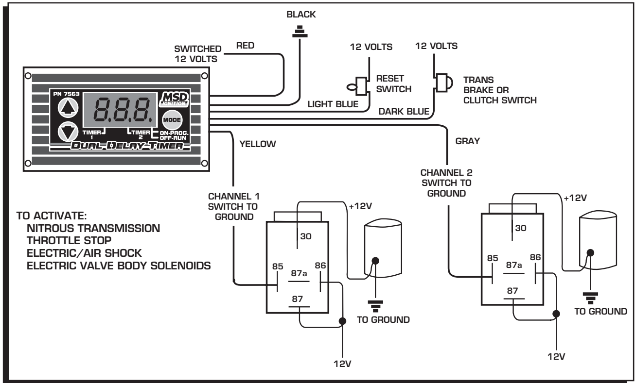
Figure 3 Wiring High Current Applications Switching to +12V.
