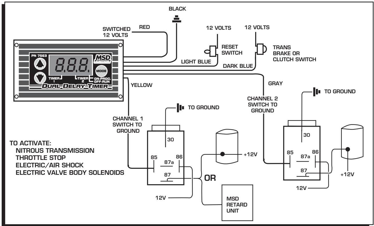
Figure 4 Wiring High Current Applications Switching to Ground.
